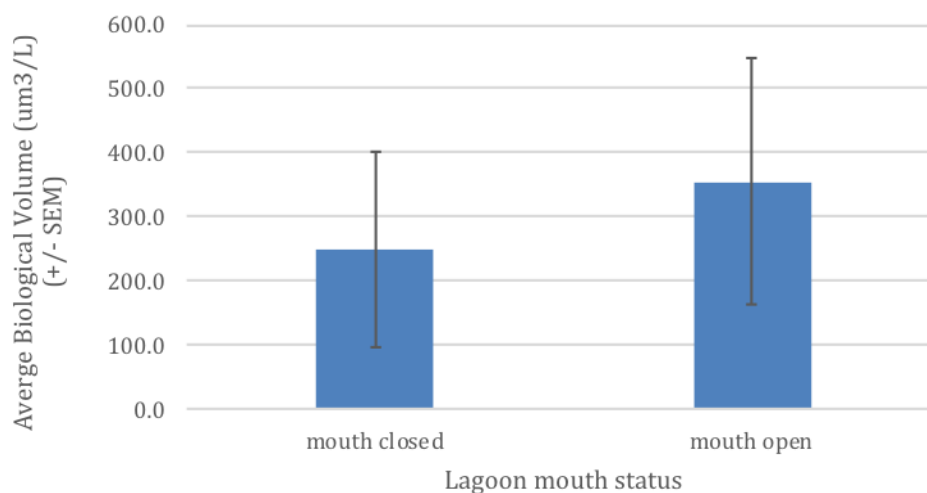
Figure 14. Average biological volume of phytoplankton (+/- Standard Error of the Mean) at Scott Creek Estuary when the mouth is open and closed from 2003-2005 (data from Beck et al. 2006). See Appendix 2 for more information.
