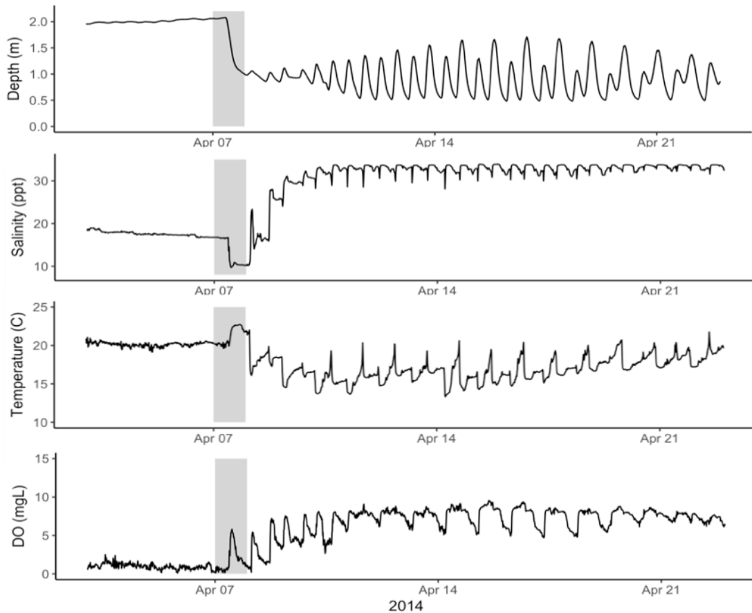
Figure 7. Managed breach event (grey bar) in Los Peñasquitos Lagoon, April 2014 (Los Peñasquitos Lagoon Foundation (2016)). Top panel: water level. Second panel: salinity near-bottom. Third panel: temperature near-bottom. Bottom panel: dissolved oxygen near-bottom.
