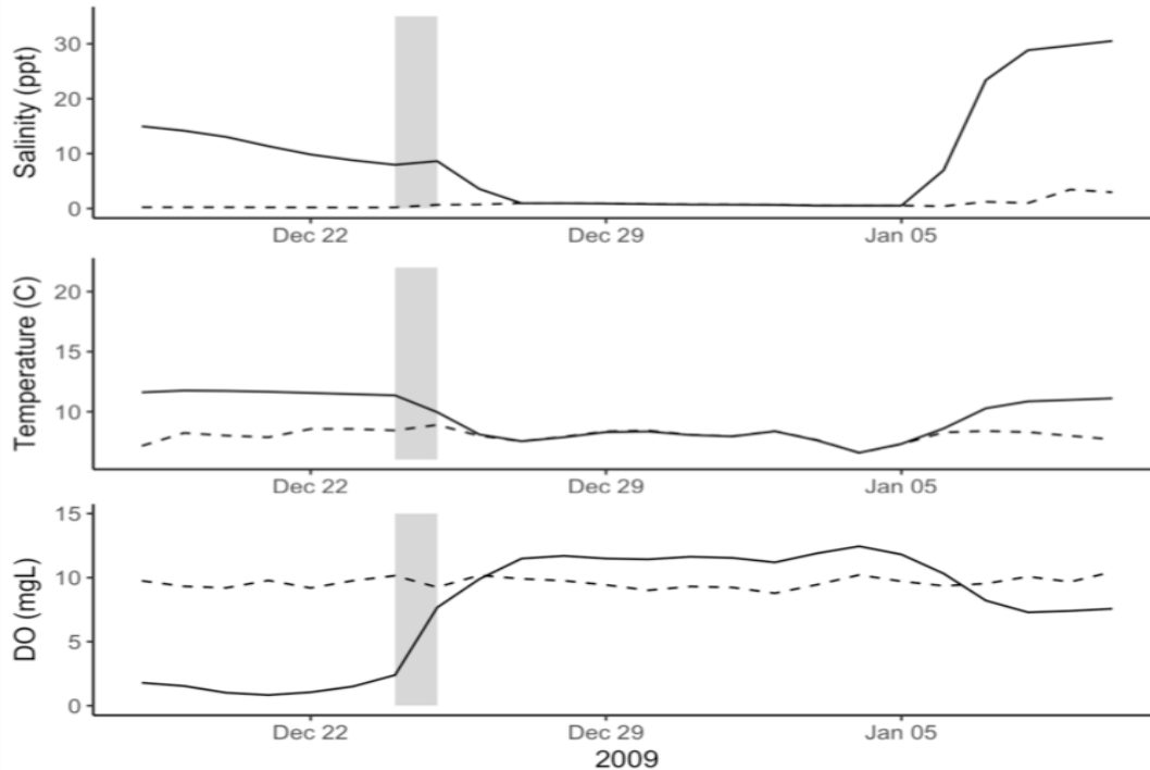
Figure 8. Natural breach event (grey bar) in Scott Creek Estuary, December 2009 (Nylen 2015). Top panel: daily average salinity near-surface (dashed line) and near-bottom (solid line). Middle panel: daily average temperature near-surface (dashed line) and near-bottom (solid line). Bottom panel: daily average dissolved oxygen near-surface (dashed line) and near-bottom (solid line).
